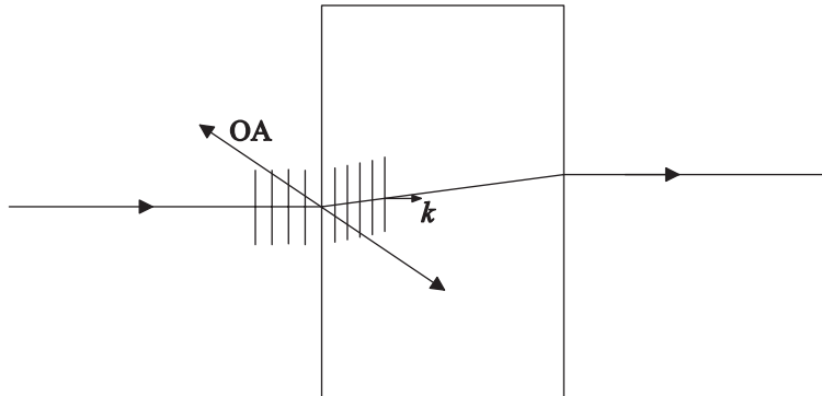
Figure 3.10: The wave fronts and the k -vector for the e-wave.
