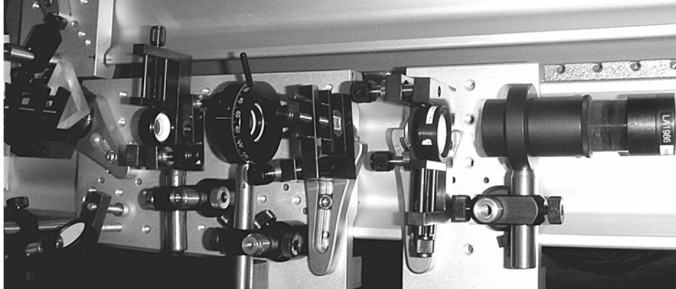
Picture 4.1: Photograph of the experimental setup.
