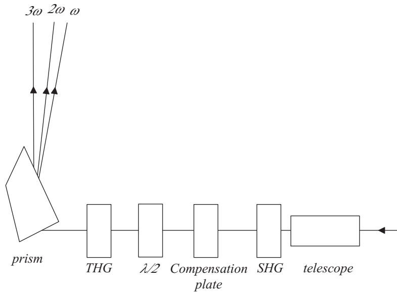
Figure 4.1: Schematic view of the experimental setup.
