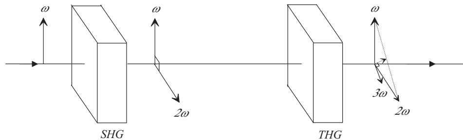
Figure 3.2: Simple setup for THG.
