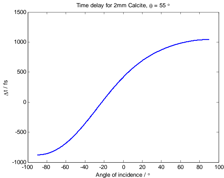
Figure 3.14: Example curve for a Calcite compensation plate.
