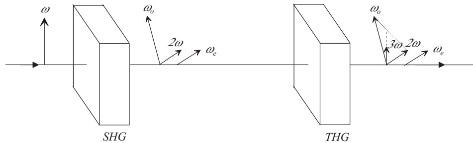
Figure 3.3: Simple THG with type 2 SHG.
