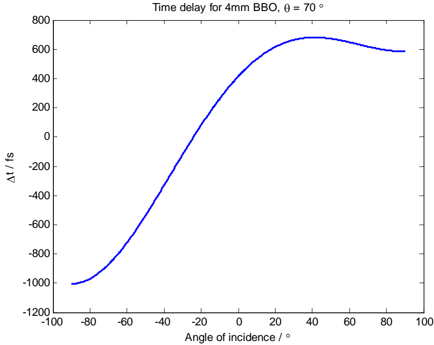
Figure 3.13: Example curve for a BBO compensation plate.
